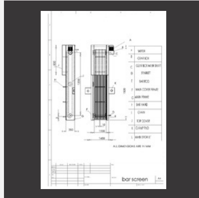
Automatic Bar Screen
